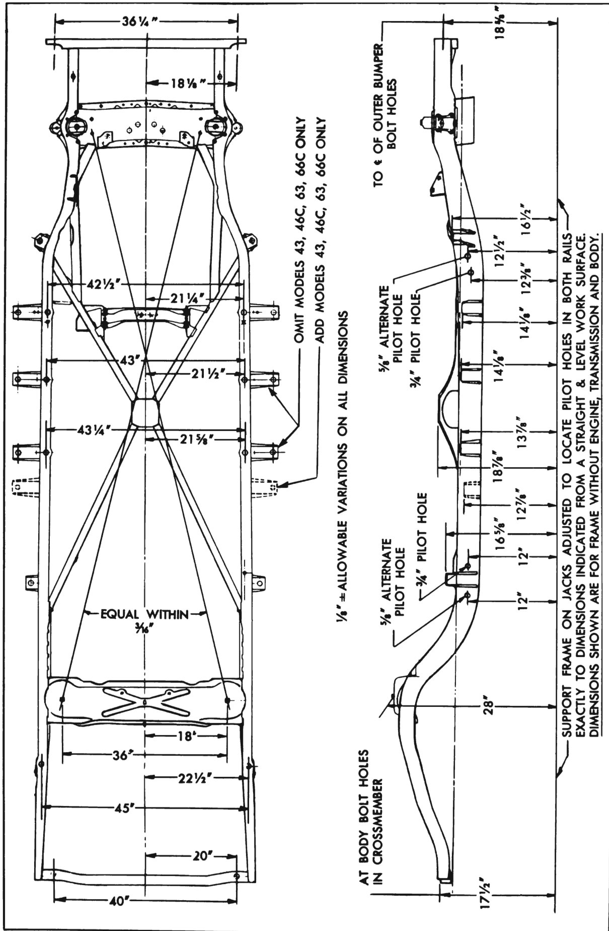
Figure 12-2—Frame Checking Dimensions—Series 40-60
