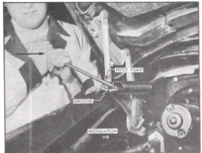
Figure 12-7—Installation of Hood Spring
