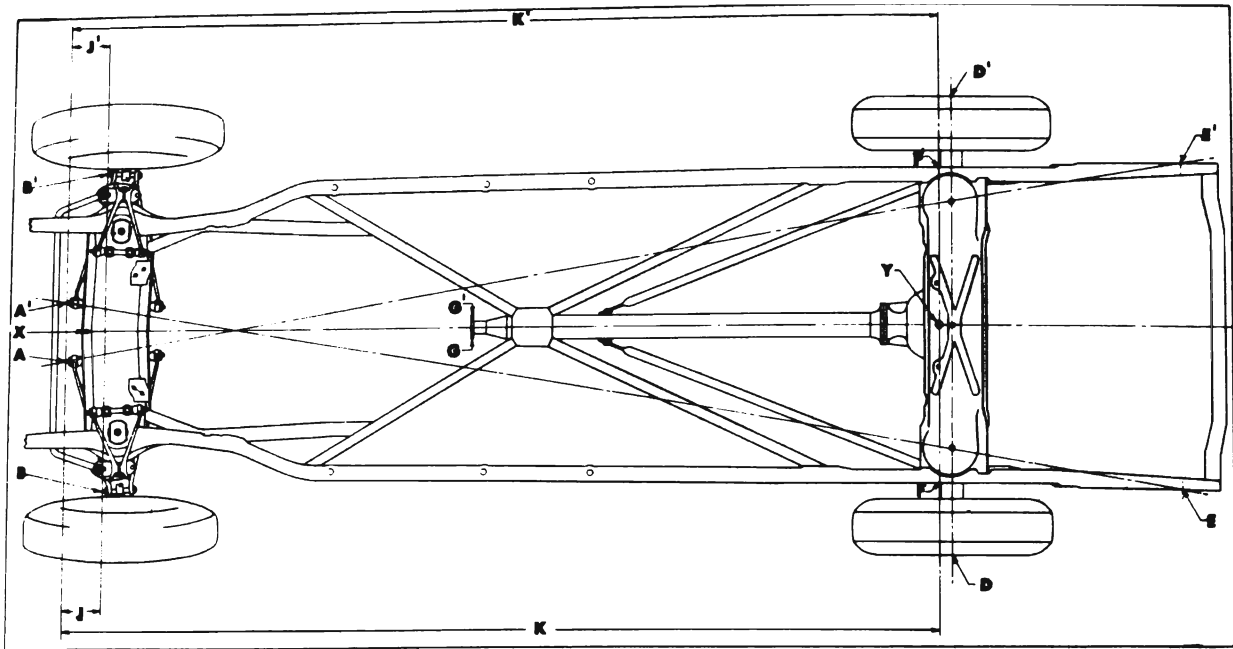
Figure 12-1—Checking Points for Frame and Suspension Alignment
