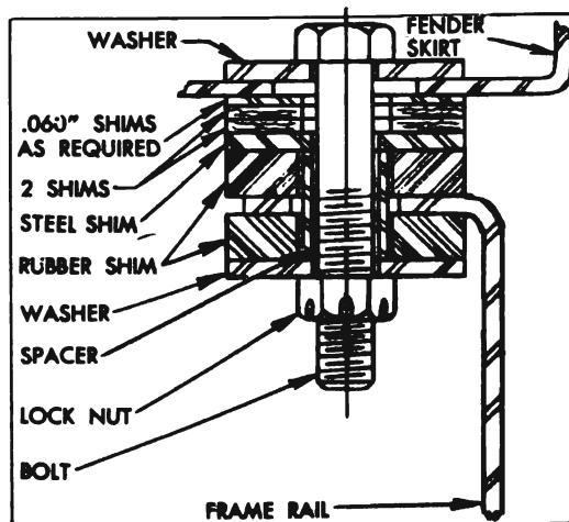
Figure 12-5—Fender Skirt Mounting Bolt and Shims
