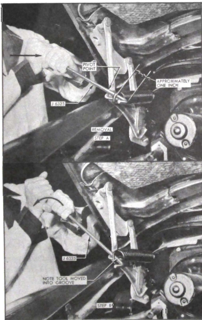
Figure 12-6—Removal of Hood Springs
